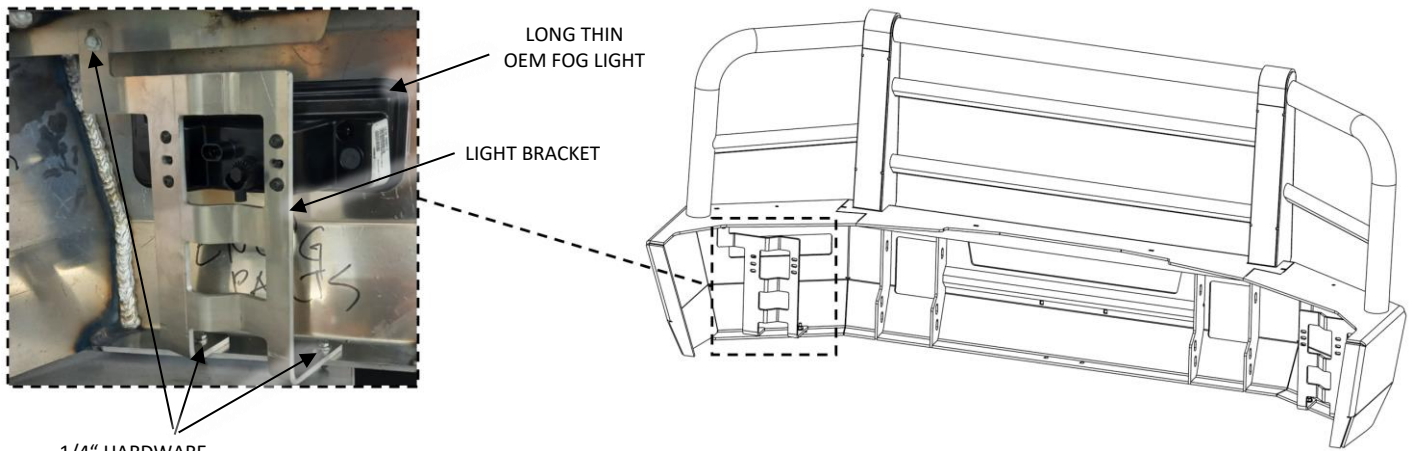
Figure 3d: Long Thin OEM Fog Light installation (Driver Side shown)
