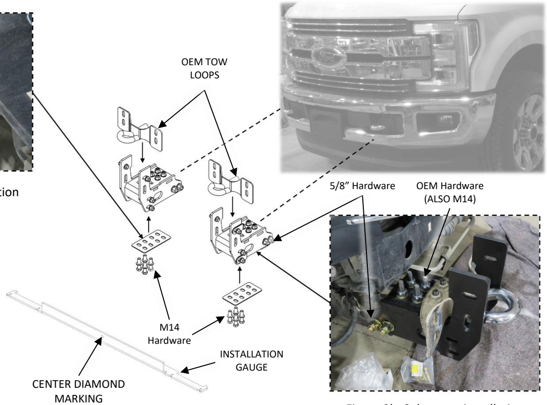
Figure 2b: Submount installation
