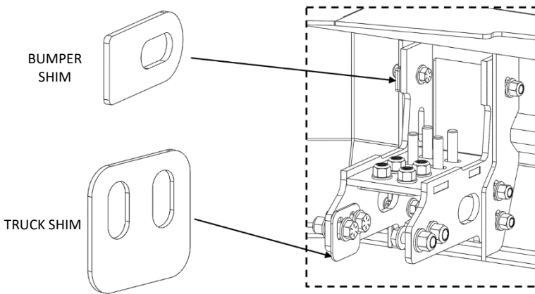
Figure 3b: Truck Guard installation (Driver Side shown)
