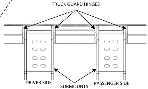
Figure 3c: Submounts position
